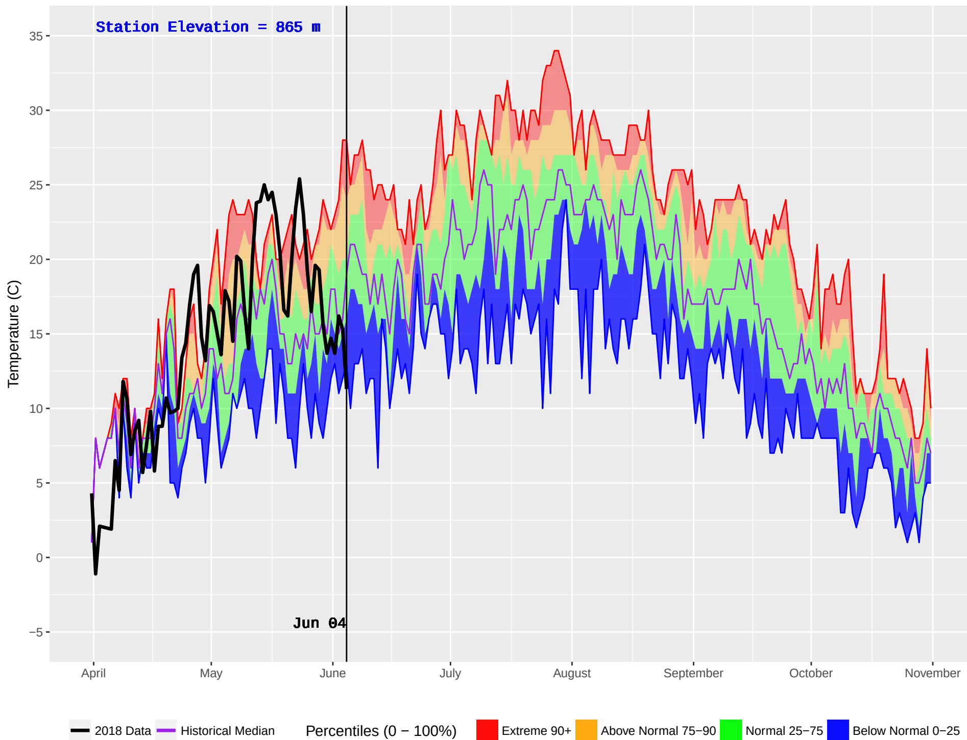
FIVE MILE (1029) : Historical (2008–2016) and Current (2018) Noon Temperature
