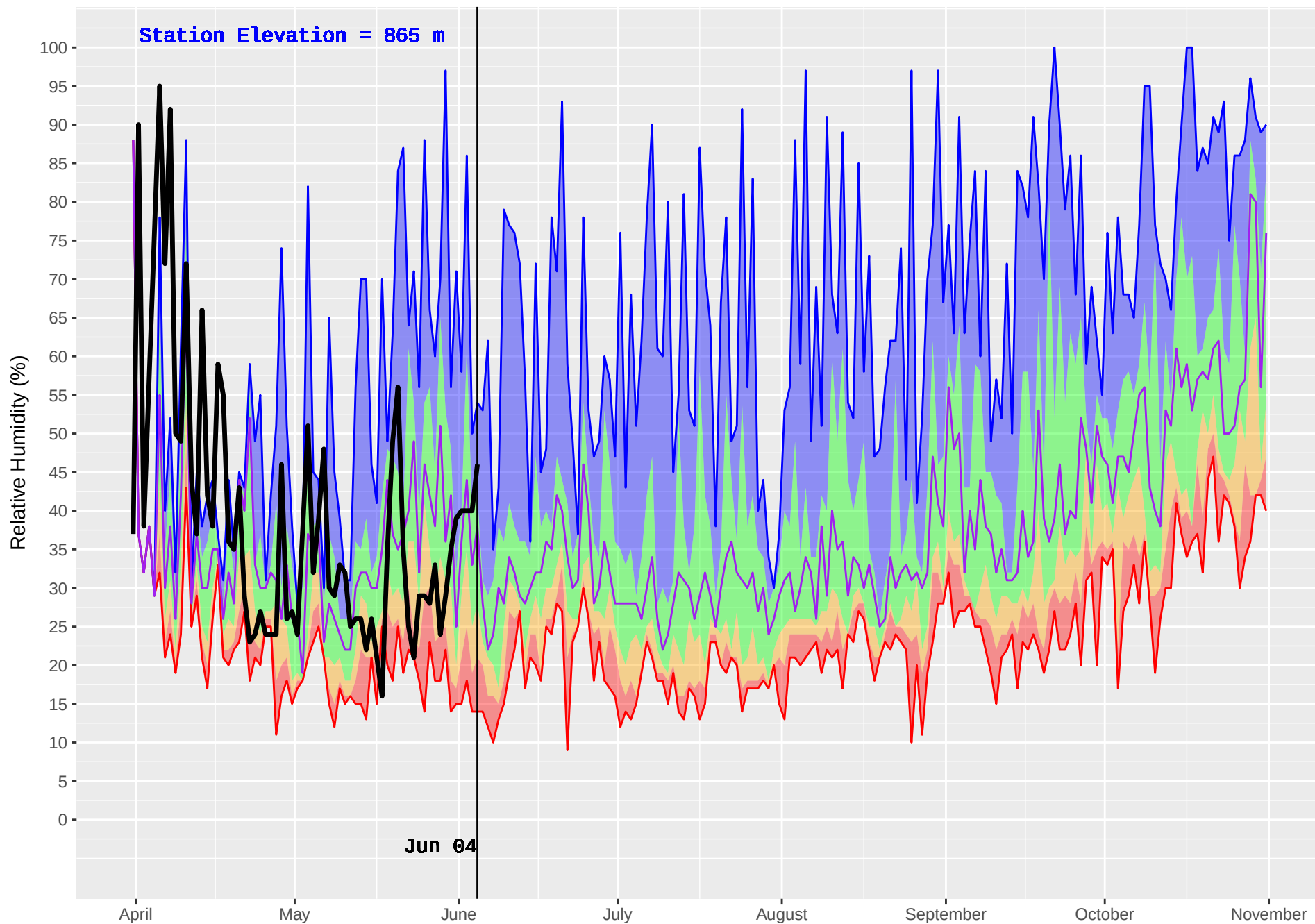
FIVE MILE (1029) : Historical (2008–2016) and Current (2018) Noon Relative Humidity
