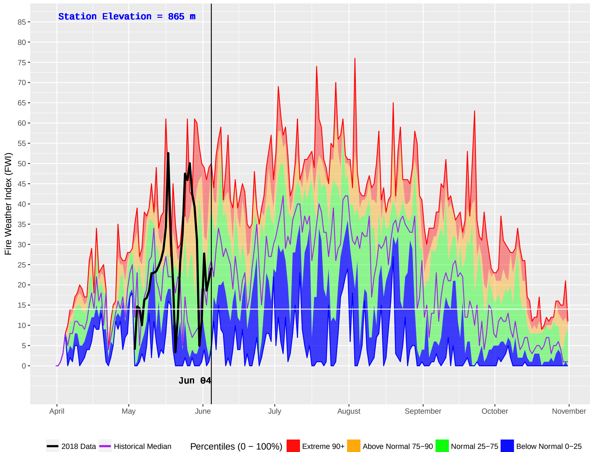
FIVE MILE (1029) : Historical (2008–2016) and Current (2018) Noon Fire Weather Index (FWI)
